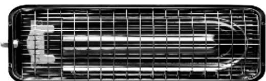
Fig 3. Aniheater comes in 3 variants 100-150-175 Watt. Available with 2.4 m cable. Certifications: IP X9K.
